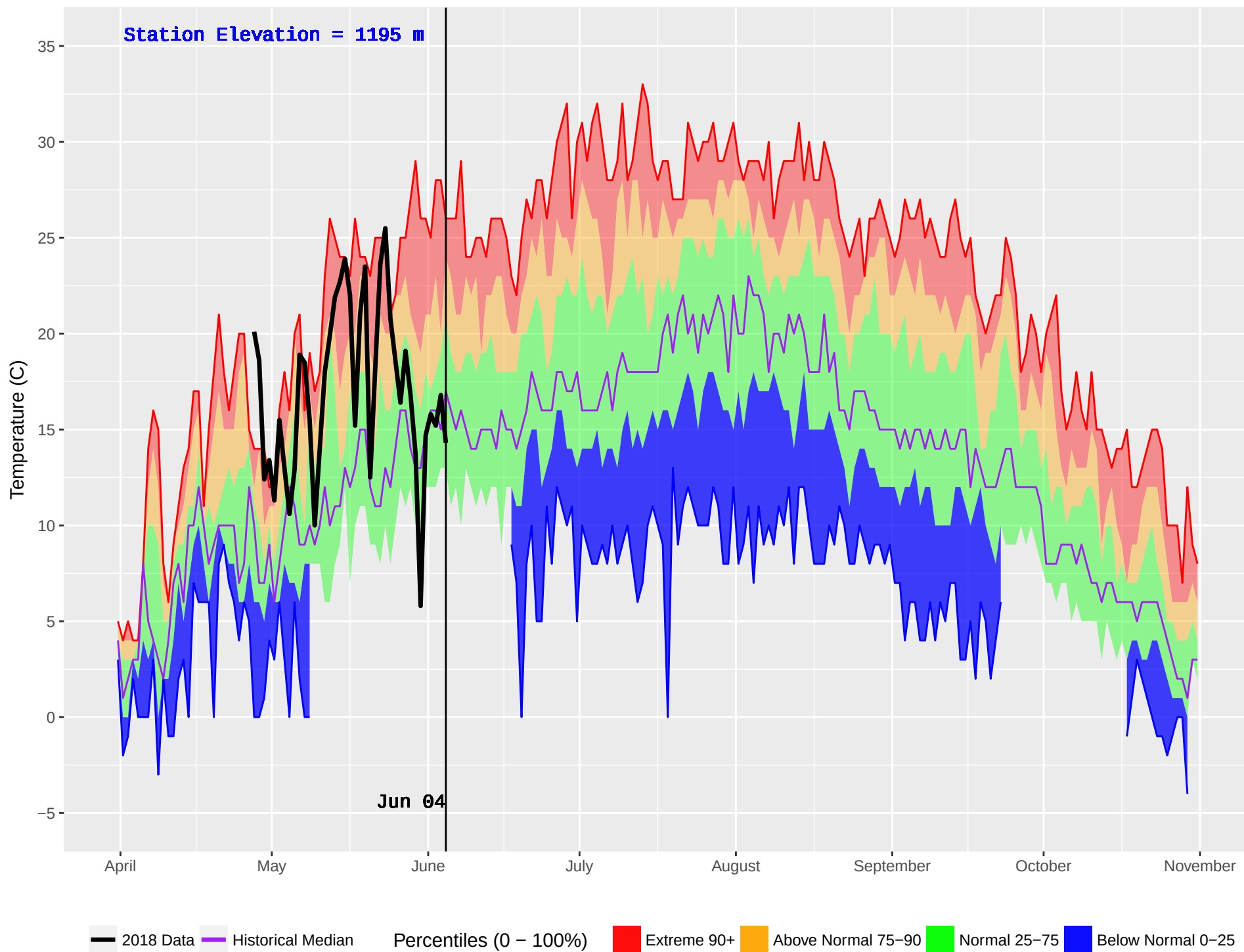
VALEMOUNT 2 (200) : Historical (1986–2016) and Current (2018) Noon Temperature
