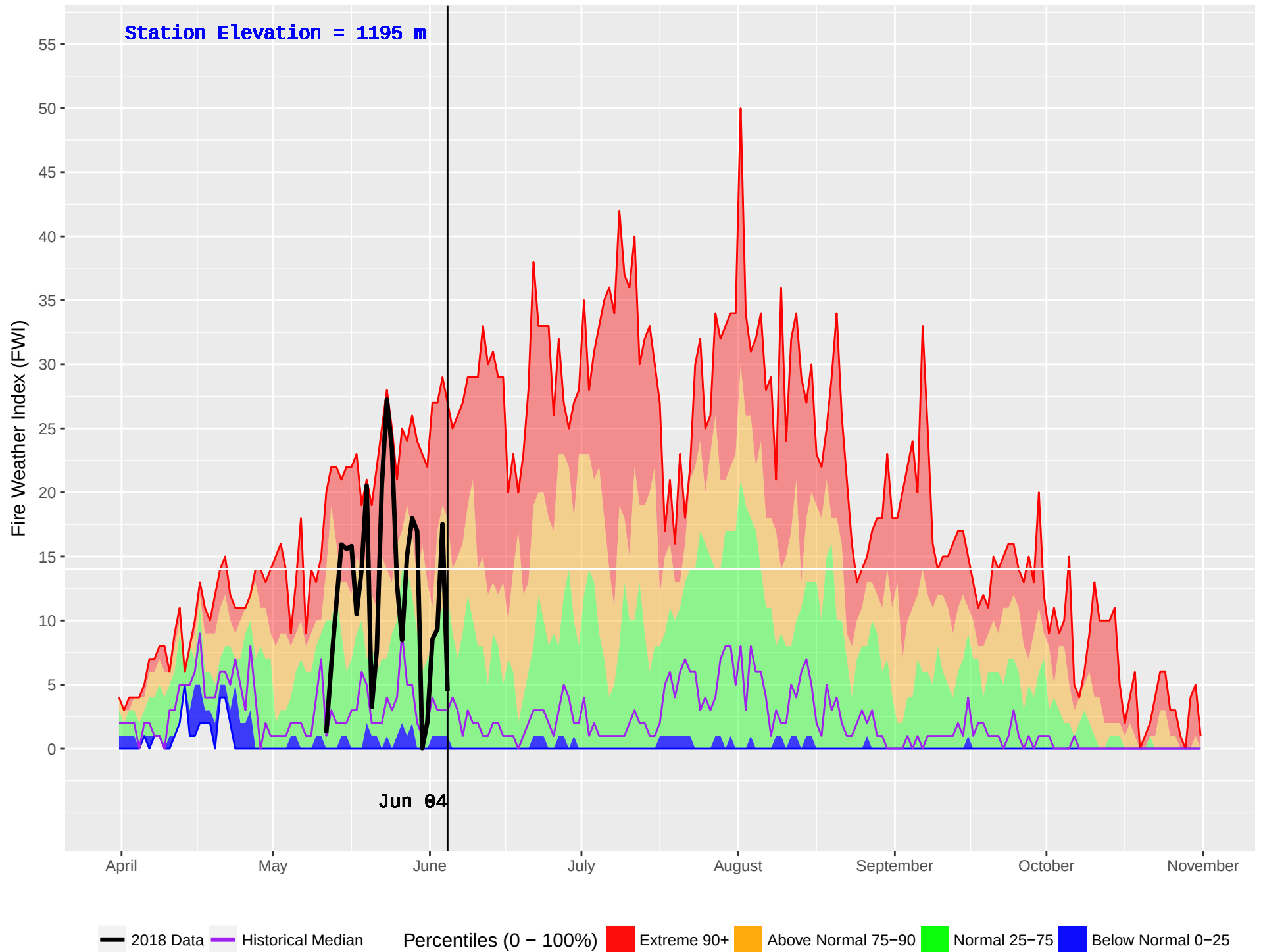
VALEMOUNT 2 (200) : Historical (1986–2016) and Current (2018) Noon Fire Weather Index (FWI)
