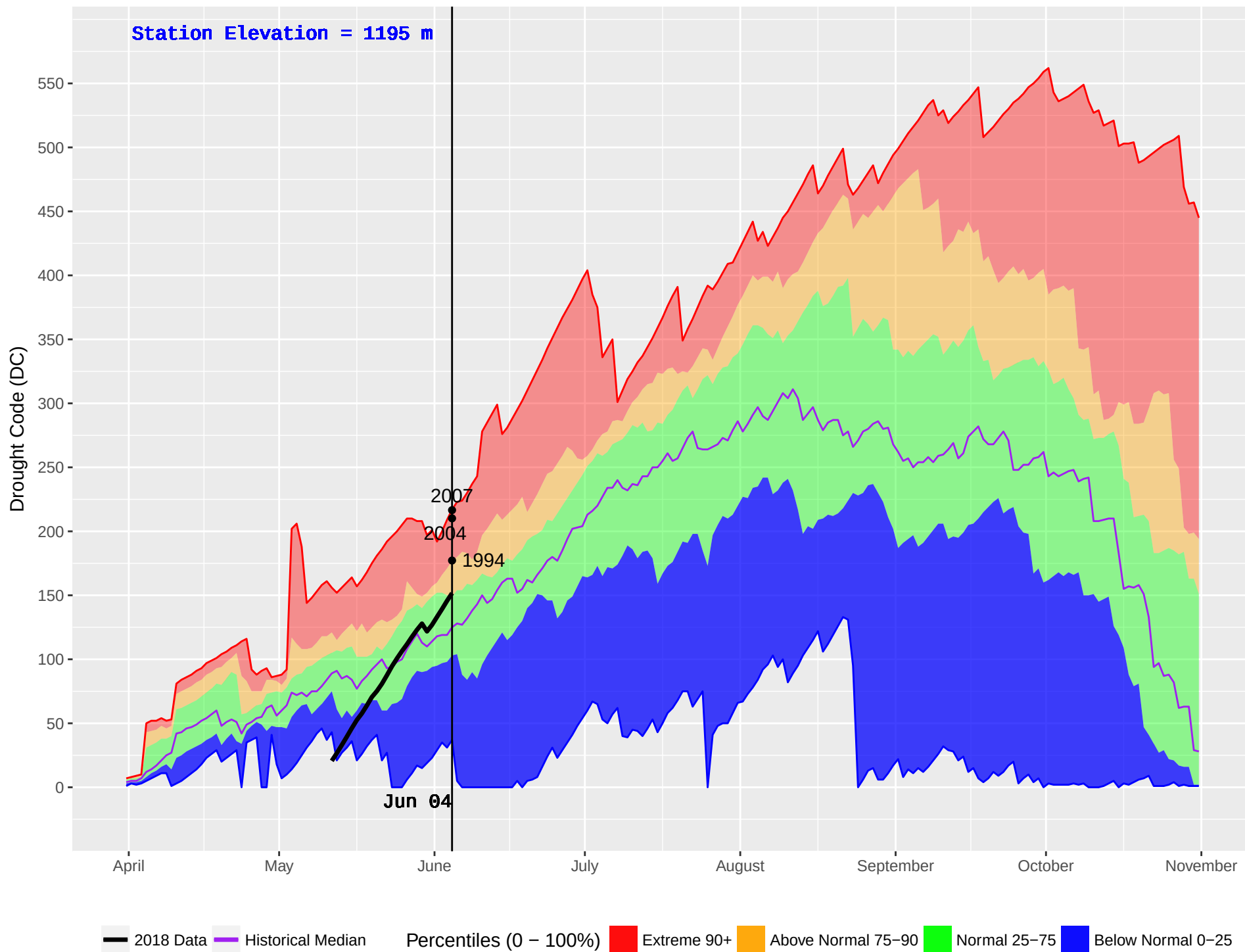
VALEMOUNT 2 (200) : Historical (1986–2016) and Current (2018) Noon Drought Code (DC)
